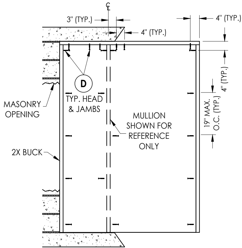
BUCK ANCHORING
