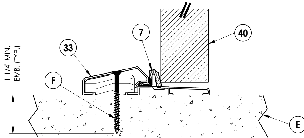
5 7 VERTICAL CROSS SECTION Shown w/ ADA threshold
