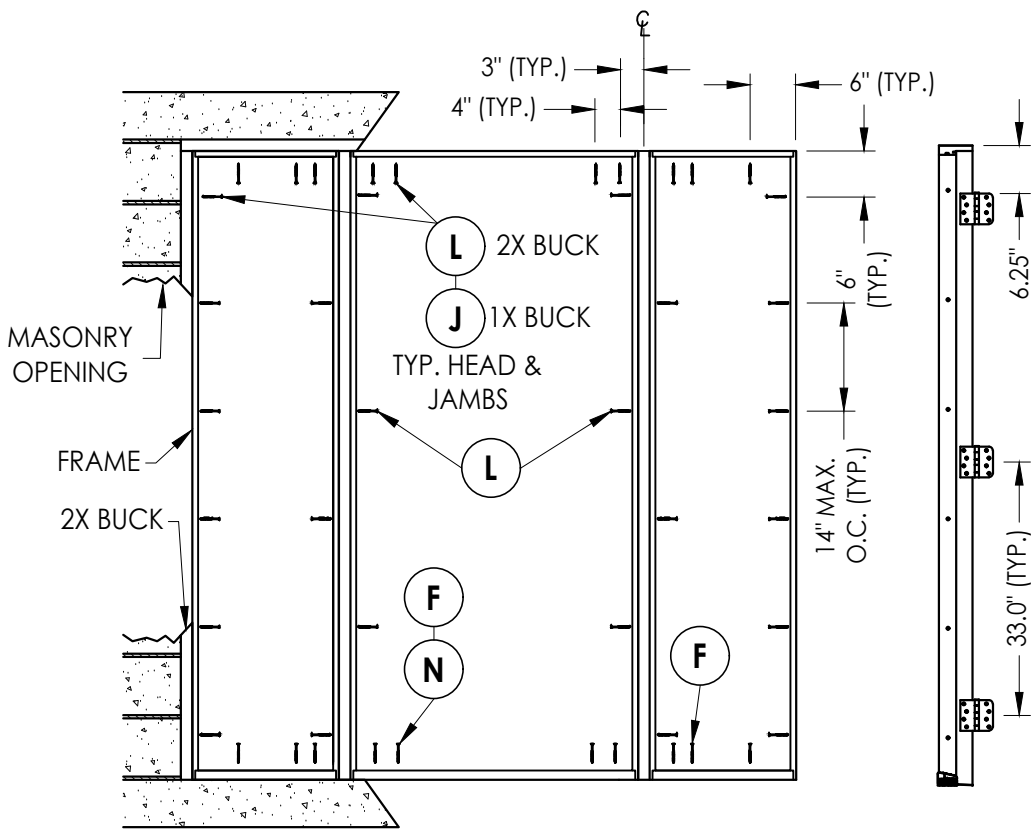
FRAME ANCHORING Masonry construction
