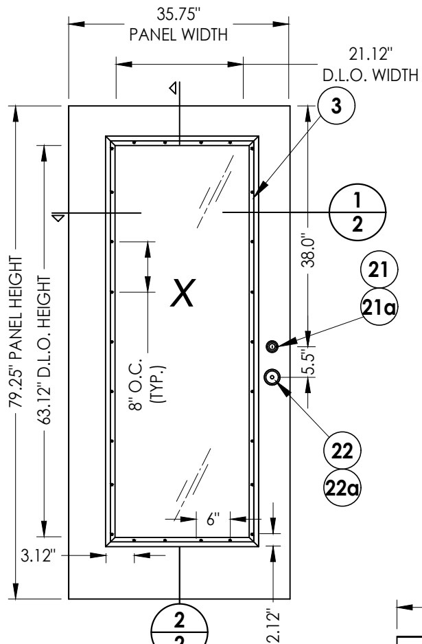
40 DOOR PANEL Fiberglass
