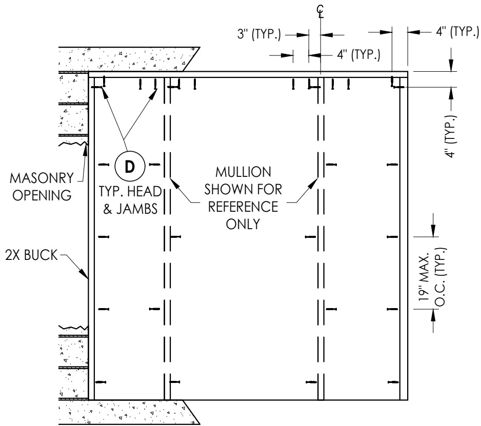
BUCK ANCHORING
