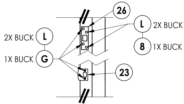
LATCH & DEADBOLT DETAIL SECURITY STRIKE
